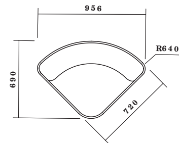
CIR-M-1030-LB/HB WITH LOW - OR - HIGH PRIVACY SCREEN
