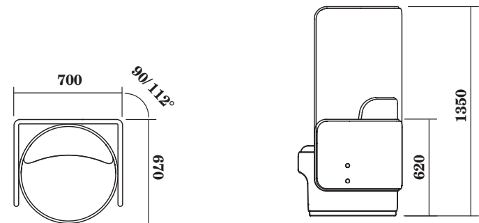
CIR-L-1010-LB/HB WITH LOW - OR - HIGH PRIVACY SCREEN
