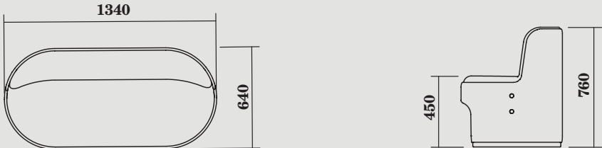
CIR-L-2010 WITH LOW - OR - HIGH PRIVACY SCREEN
