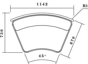
CIR-M-1040-LB/HB WITH LOW - OR - HIGH PRIVACY SCREEN
