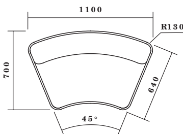
CIR-M-1040 CIRCOLO MODULAR - SINGLE SEAT - 45DEG CURVE
