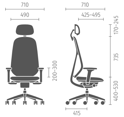
High backrest 4D armrests and neck support
