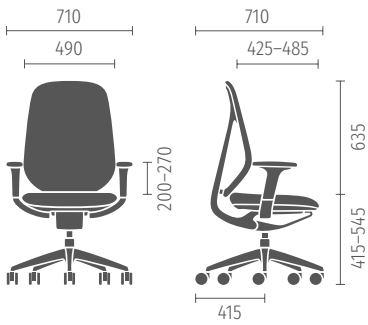
Medium backrest 2D design armrests
