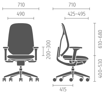
Medium height-adjustable backrest 4D armrests
