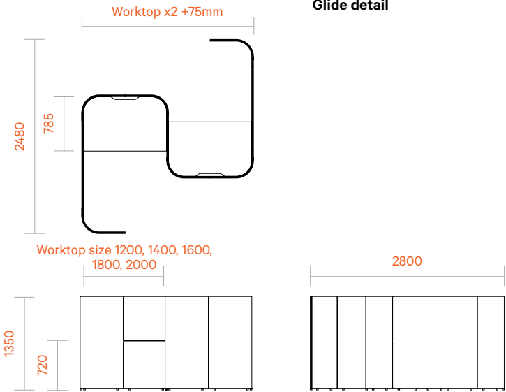
Glide detail
